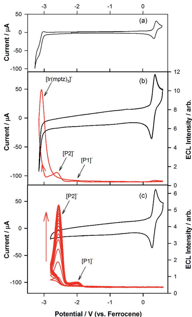
Fig. 2 (a) Cyclic voltammogram at a scan rate of 0.1 \text{V s}^{-1} for 0.5 mM \text{Ir}(\text{mptz})_3 in acetonitrile containing 0.1 M \text{TBAPF}_6 . (b) Cyclic voltammogram in the range of 0.6 V and -3.2 V versus \text{Fc}^+/\text{Fc} at 0.1 \text{V s}^{-1} overlaid with the ECL signal detected using a PMT. (c) Cyclic voltammogram overlaid with the ECL signal in the range of 0.6 V and -2.8 V versus \text{Fc}^+/\text{Fc} at a scan rate of 1.0 \text{V s}^{-1} .
