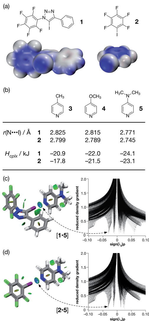
Fig. 2 (a) Calculated electrostatic potential surfaces for compounds 1 and 2 (TPSSh/def2-TZVP). Colour scale: positive (blue = +0.08) → neutral (white) → negative (red = -0.08). (b) Calculated pyridine ring N...I distances and interaction energies ( H_{\text{cplx}} , TPSSh/def2-TZVP enthalpies of complexation at 298 K, see ESI† for details) for a series of complexes between halogen bond donors 1 and 2 and pyridine-based acceptors. Visualisation of the interaction between 4-(dimethyl amino) pyridine 5 and (c) compound 1 and (d) compound 2 . Left: intermolecular interaction isosurfaces generated by NCIPLOT 26 for s = 0.5 and -0.05 < \text{sign}(\lambda_2)\rho < 0.05 (colour scale: attractive (blue) → repulsive (red)). Right: plots of \text{sign}(\lambda_2)\rho vs. reduced density gradient highlighting the favourable interaction corresponding to the halogen bond at \text{sign}(\lambda_2)\rho \sim -0.035 . Atom colouring: C atoms = grey, N atoms = blue, O atoms = red, F atoms = light green, I atoms = purple.
