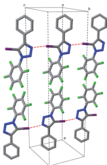
Fig. 1 Solid state structure of diaryl-5-iodo-1,2,3-triazole 1 determined from single crystal X-ray diffraction data. Potential halogen bonds are marked in red ( r(\text{N}\cdots\text{I}) = 2.973 \text{ \AA} ; \angle \text{C}-\text{I}\cdots\text{N} = 168.9^\circ ). Atom colouring: C atoms = grey, N atoms = blue, F atoms = light green, I atoms = purple. Hydrogen atoms are omitted for clarity.
