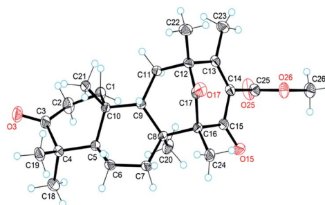
Fig. 2 X-ray crystal structure of asperterpene A ( 1 ).
