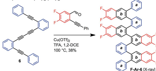
Scheme 2 Synthesis of sequence-defined ortho -arylene oligomers from ortho -arylethyneynes via a cycloaddition strategy.
