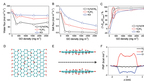
Fig. 7 Concentration gradient-driven water and salt diffusions through GOLM on a microfilter with increased GO coverage density. (A) Water fluxes, (B) salt fluxes and (C) nominal rejections. Feed concentration of salts: 0.1 M; feed concentration of D_2O : 30 wt%. (D and E) Atomic structures of GO sheets that defined a finite-length channel for ion and water diffusions in SMD simulations. (F) Free energy profiles for water and ion ( K^+ and Cl^- ) transport across the channel obtained from SMD simulations.
