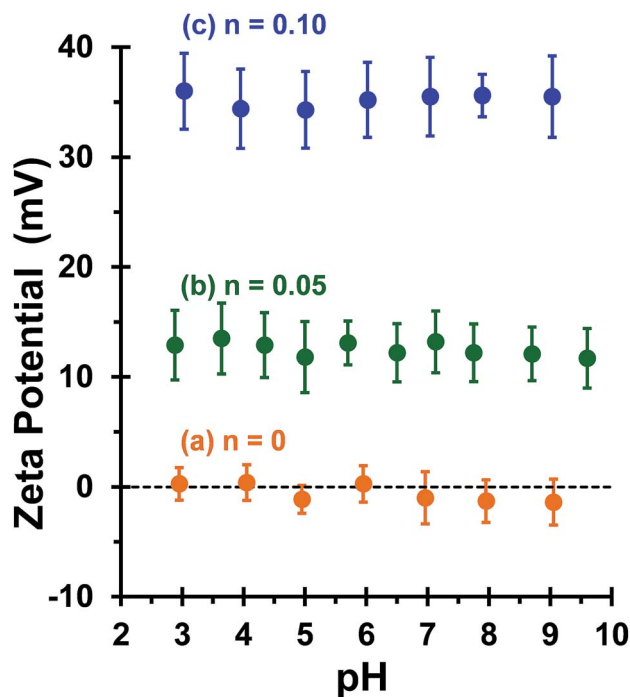
Fig. 2 Zeta potential vs. pH curves obtained for a series of ([1 - n] \text{ PEO}_{113} + n\text{PQDMA}_{125})\text{-PHPMA}_{225} linear diblock copolymer worms prepared at 20% w/w solids by the RAFT aqueous dispersion polymerization of HPMA at 50 °C, where (a) n = 0 , (b) n = 0.05 and (c) n = 0.10 . Zeta potentials were determined at 20 °C for 0.1% w/w copolymer dispersions in the presence of 1 mM KCl. Error bars are equivalent to one standard deviation. The aqueous dispersion pH was adjusted using either 0.1 M or 1 M HCl.
