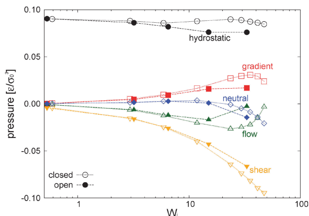
Fig. 12 Hydrostatic pressure and components of the traceless stress tensor obtained in closed and open domains at fixed T = 4 and under the adpd thermostat (normal friction). Error bars of the measured quantities are approximately 0.005\epsilon/\sigma_0^3 .
