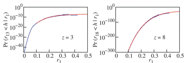
Fig. 5 Extrapolating the zero distance probability G_{12}(h|r_1) (blue lines) using eqn (27) (red lines). G_{12}(h|r_1) \equiv \text{Pr}(r_{12} < h|r_1) is the probability that a pore with radius r_1 will have exactly z contacts with real particles in a shell of width h . The data represent 39 combined fluidized bed packings (Q_150) with an average \phi of 0.585. The particle diameter is normalized to unity, the extrapolation is therefore to r_1 = 0.5 .
