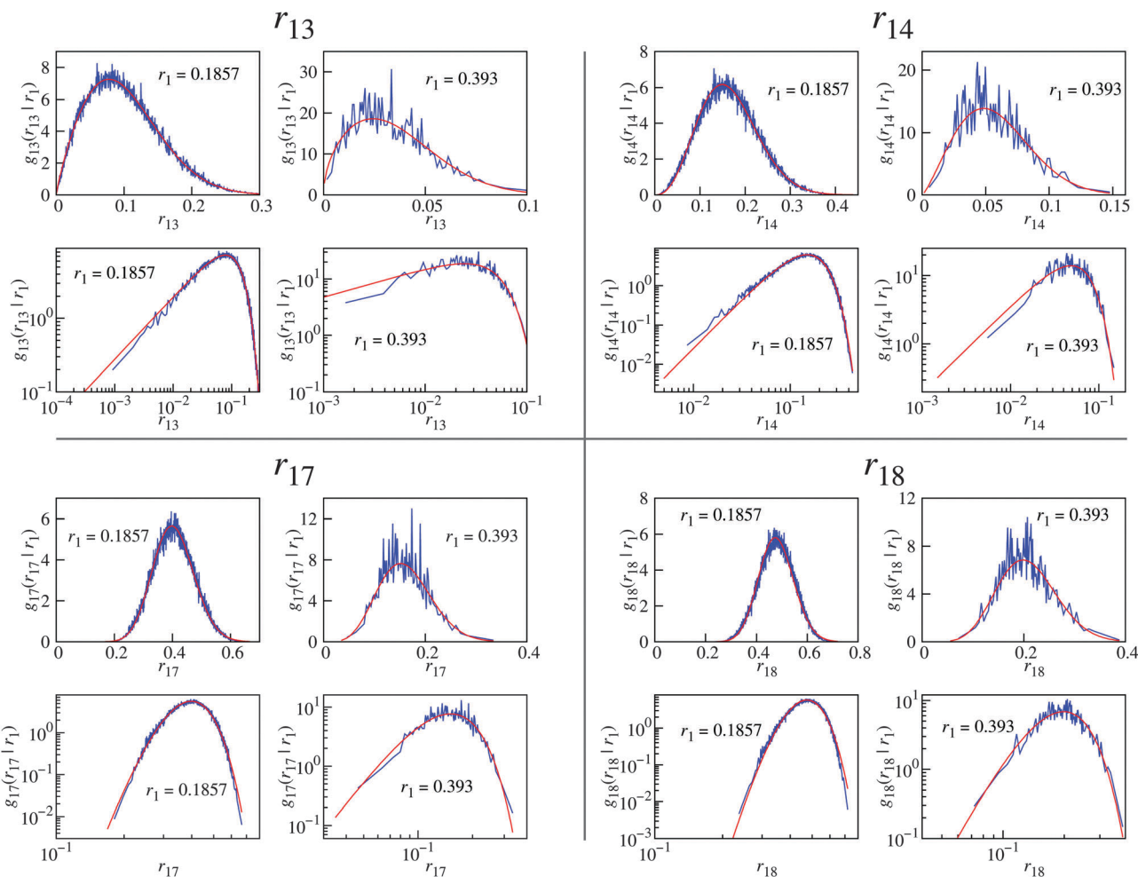
Fig. 4 The experimentally obtained g_{12}(r_{12}|r_1) (blue lines) are fit well with Nakagami distributions (red lines). The data represent 39 combined fluidized bed packings (Q_150) with an average \phi of 0.585. Distributions for r_{13} , r_{14} , r_{17} , and r_{18} (respectively z = 3, 4, 7 , and 8 ) are displayed. Each fit is shown twice, in a linear (top) and in a log-log scale (bottom). The particle diameter is normalized to unity.
