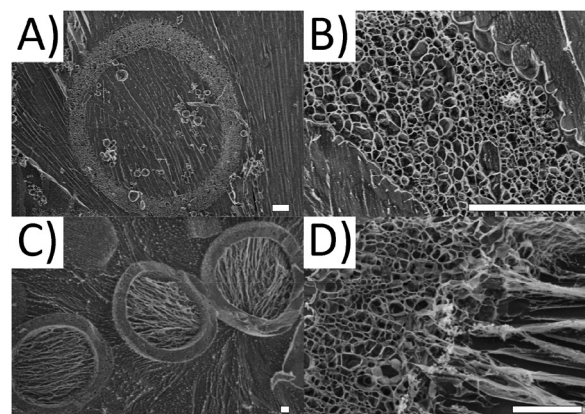
Fig. 4 Cryo-SEM images of the microgel capsules: samples are purified and stored in Milli-Q water. (A) 10 minutes sublimation time at -80 \text{ }^{\circ}\text{C} , 700x; (B) 10 minutes sublimation time at -80 \text{ }^{\circ}\text{C} , 5000x; (C) 25 minutes sublimation time at -80 \text{ }^{\circ}\text{C} , 400x; (D) 25 minutes sublimation time at -80 \text{ }^{\circ}\text{C} , 3000x. Scale bars are 10 \mu\text{m} .
