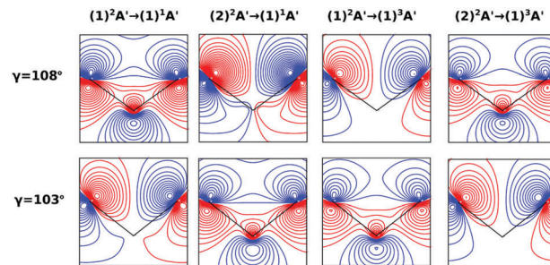
Fig. 7 Dyson orbitals in the zx plane at r_a = 0 Å and \gamma = 108^\circ (top) and \gamma = 103^\circ (bottom). The initial and final states of the photoionization process for each column are shown at the top of the figure.
