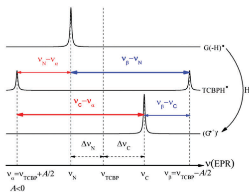
Scheme 1 Schematic representation of triplet-singlet interconversion based on the EPR spectra of G(H) \cdot (top), TCBPH \cdot (middle), and (G \cdot )' (bottom). Only a single spin-1/2 nucleus in TCBPH \cdot with negative HFCC is considered.
