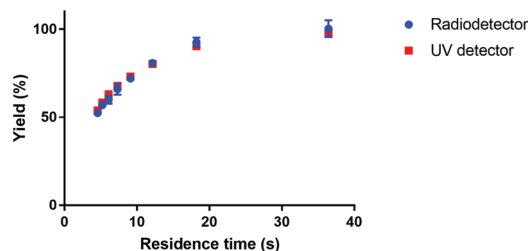
Fig. 3 Comparison of measured reaction yield of ^{177}\text{Lu} -Lu-DOTA-TATE for UV and radio-detection. The reaction was done in a 100 \mu\text{m} channel at 80 \text{ }^\circ\text{C} .
