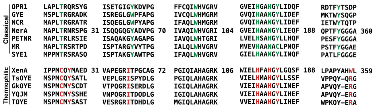
Fig. 1 Sequence alignment, using PROMALS3D, 23 showing selected regions covering the active site residues of 'classical' and 'thermophilic-like' class of OYEs. Active site residues are highlighted in green and red for classical and thermophilic-like OYEs respectively. Residue numbers are displayed for NerA and XenA.
