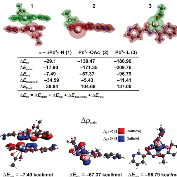
Fig. 9 (Top) Cluster models of [PbL(OAc)] 2 together with the fragmentation patterns 1–3 together with the fragmentation patterns 1–3 applied in the ETS-NOCV analysis. (Bottom) The overall deformation densities \Delta\rho_{orb} of 1–3 with the corresponding energies \Delta E_{orb} .
