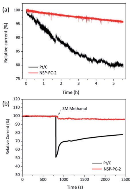
Fig. 6 (a) The durability of the catalyst-modified electrodes for the ORR in oxygen-saturated 0.1 M KOH. (b) i – t chronoamperometric responses of the catalyst-modified electrodes at 0.6 V (vs. RHE) with a rotating speed of 1600 rpm in oxygen-saturated 0.1 M KOH. The arrow indicates the addition of methanol into the electrolytic cell.
