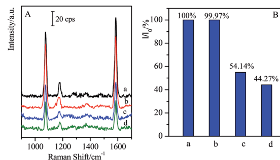
Fig. 7 Comparison of SERS spectra based on competitive immunoassay by non-specific and specific separation. (a) Blank; (b) separated by (\text{Fe}_3\text{O}_4@Au)\text{-CL}_{ab} ; (c) separated by (\text{Fe}_3\text{O}_4@Au)\text{-SAL}_{ab} ; (d) 1 \text{ ng mL}^{-1} of CL without separation.
