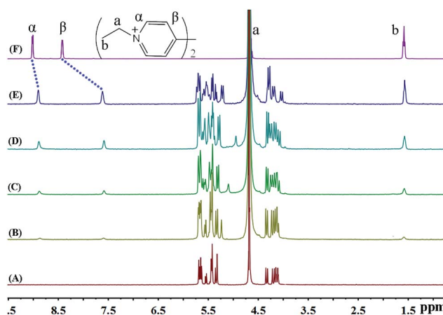
Fig. 3 ^1\text{H} NMR spectra (400 MHz, D _2 O) of iQ[7] (A) in the absence and in the presence of (B) 0.1, (C) 0.3, (D) 0.5, (E) 1.0 equivalent of EV ^{2+} and (F) neat EV ^{2+} in D _2 O at 20 °C.
