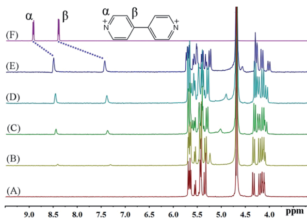
Fig. 1 ^1\text{H} NMR spectra (400 MHz, D _2 O) of iQ[7] (A) in the absence and in the presence of (B) 0.2, (C) 0.4, (D) 0.8, (E) 1.1 equivalents of BPY ^{2+} and (F) neat BPY ^{2+} in D _2 O at 20 °C.
