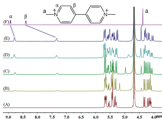
Fig. 2 ^1\text{H} NMR spectra (400 MHz, D _2 O) of iQ[7] (A) in the absence and in the presence of (B) 0.1, (C) 0.4, (D) 0.8, (E) 1.1 equivalents of MV ^{2+} and (F) neat MV ^{2+} in D _2 O at 20 °C.
