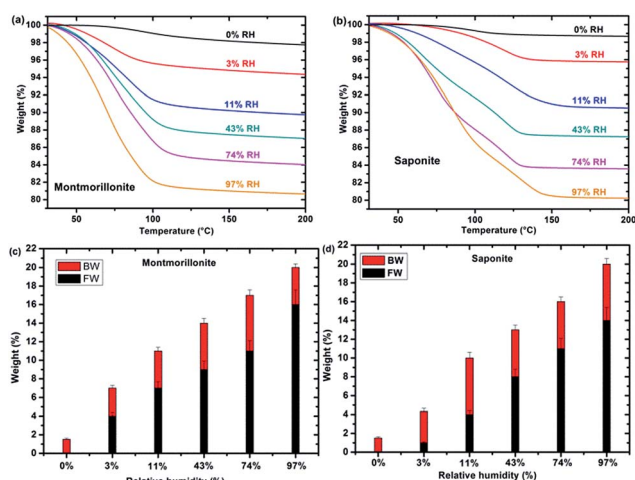
Fig. 2 TGA from 30 to 200 ^{\circ}\text{C} of synthetic montmorillonite (a) and saponite (b) according to relative humidity (upper part). Free Water (FW, in black), Bonded Water (BW, in red) and Total Water Content (TWC) (in weight percent) are represented for synthetic montmorillonite (c) and saponite (d) (lower part).
