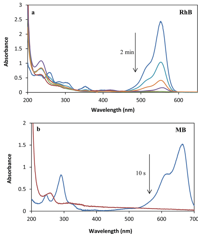
Fig. 17 UV-Vis spectra of reduction of (a) RhB ( 2.1 \times 10^{-5} M) and (b) MB ( 3.1 \times 10^{-5} M) with [\text{NaBH}_4] = 2.6 \times 10^{-3} M in presence of Ag/almond shell nanocomposite = 5.0 mg.
