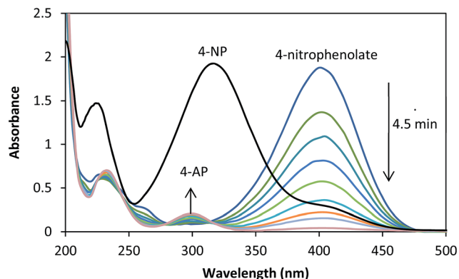
Fig. 16 UV-visible spectra for catalytic reduction of 4-NP to 4-AP at several interval, conditions: [4\text{-NP}] = 2.5 \times 10^{-3} M, [\text{NaBH}_4] = 0.25 M, Ag/almond shell = 5.0 mg.
