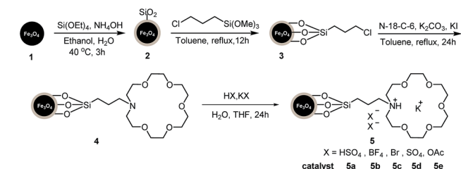
Scheme 1 Synthetic route for the magnetic core-shell particle supported aza-crown ether complex cation ionic liquids.
