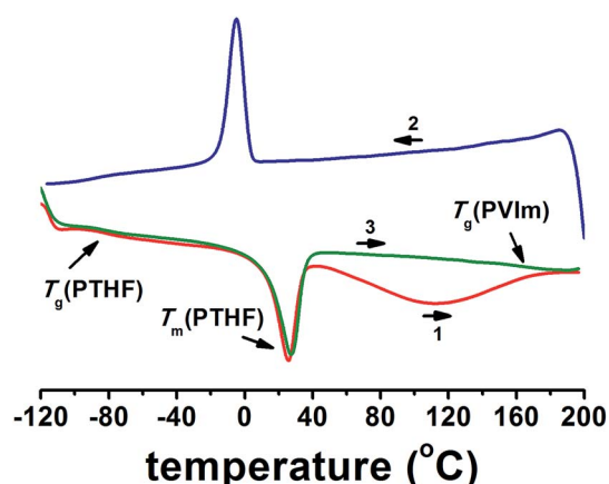
Fig. 2 Differential scanning calorimetry (DSC) thermograms (first heating (1), cooling (2) and second heating (3) cycles) of poly( N -vinylimidazole)- l -poly(tetrahydrofuran) (PVIm- l -PTHF) conetwork (P10k-62 sample; T_g(\text{PVIm}) = 158^\circ\text{C} , T_g(\text{PTHF}) = -86^\circ\text{C} , T_m(\text{PTHF}) = 27^\circ\text{C} ).
