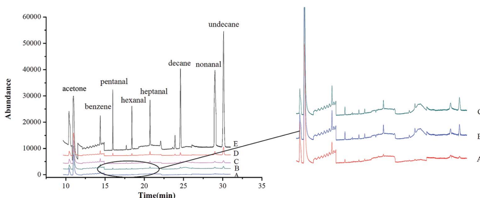
Fig. 6 GC-MS-SIM chromatograms of VOCs in EBV samples ((A) healthy volunteer, (B) lung cancer patient, (C) lung cancer cell line, (D) spiked EBV of healthy volunteer (0.5 μg L -1 ), (E) spiked EBV (5 μg L -1 )).
