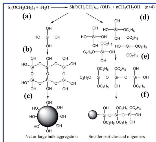
Scheme 1 Schematic illustration of hydrolysis–condensation for different H_2O/TEOS ratios, where (a) and (d) present the progress of hydrolysis, (b) and (e) show the progress of condensation, and (c) and (f) give the formation of silica particles.
