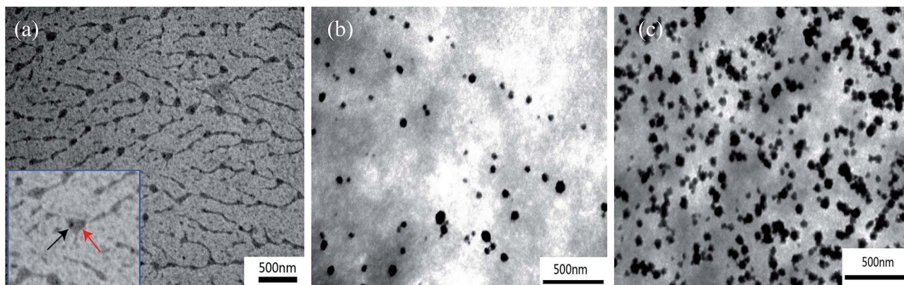
Fig. 1 TEM images of the silica/PVA hybrids obtained using different H_2O/TEOS ratios ( r ): Sample A ( r = 1 ), Sample B ( r = 4 ) and Sample C ( r = 12 ).
