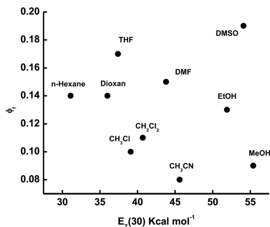
Fig. 5 Plot of \phi_{\text{f}} versus E_{\text{T}}(30) for the elected solvents.
