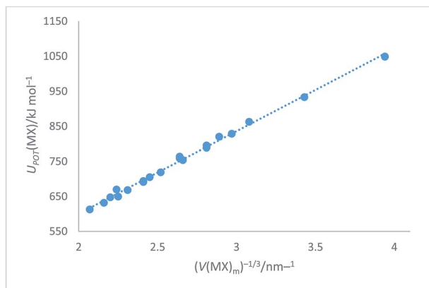
Fig. 4 Plot of U_{\text{POT}}(\text{MX})/\text{kJ mol}^{-1} as ordinate versus V(\text{MX})_m^{-1/3} as abscissa. The plot takes the analytical form: U_{\text{POT}}(\text{MX})/\text{kJ mol}^{-1} = 2I[117.8(V(\text{MX})_m)^{-1/3} + 64.5] with correlation coefficient R^2 = 0.996 , N = 20 .
