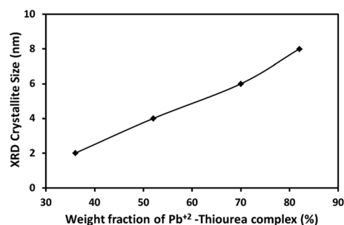
Fig. 3 Average crystallite size (Scherrer) of PbS nanoparticles in PbS/PVP nanocomposite films as a function of weight fraction of \text{Pb}^{2+} -TU complex.
