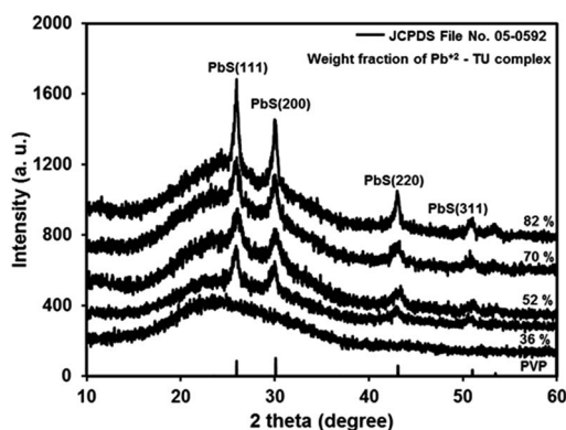
Fig. 2 X-ray diffractogram of PVP film and PbS/PVP nanocomposite films on glass with different weight fraction of \text{Pb}^{2+} -TU complex.
