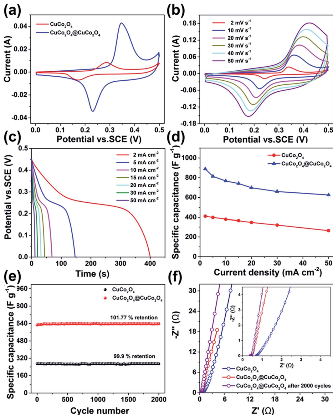
Fig. 4 (a) CV curves of the CuCo 2 O 4 and CuCo 2 O 4 @CuCo 2 O 4 electrodes obtained at a scan rate of 5 mV s -1 . (b) CV curves of the CuCo 2 O 4 @CuCo 2 O 4 electrode at various scan rates. (c) Charge–discharge curves of the CuCo 2 O 4 @CuCo 2 O 4 electrode at different current densities. (d) Specific capacitance of the CuCo 2 O 4 and CuCo 2 O 4 @CuCo 2 O 4 electrodes at different current densities. (e) Long-term cycling stability of the CuCo 2 O 4 and CuCo 2 O 4 @CuCo 2 O 4 electrodes. (f) Impedance Nyquist plots of the CuCo 2 O 4 electrode and the CuCo 2 O 4 @CuCo 2 O 4 electrode before and after 2000 cycles.
