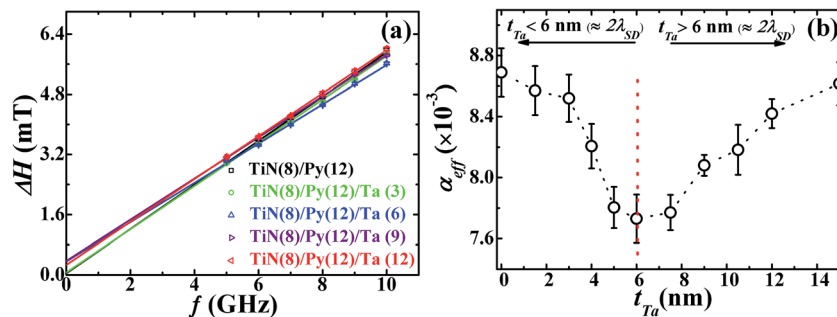
Fig. 7 (a) Variation of \Delta H with f , i.e. \Delta H vs. f at different constant t_{\text{Ta}} and the solid lines fits using eqn (5). Here the Ta layer thickness t_{\text{Ta}} varies from 1.5 to 15 nm. (b) The effective Gilbert damping constant ( \alpha_{\text{eff}} ) obtained from the fitting using eqn (5). The dotted lines are guide to the eyes. The \Delta H vs. f plots for samples with t_{\text{Ta}} = 1.5, 4, 5, 7.5, and 10.5 nm, refer Fig. 4(b) of the ESI† file.†
