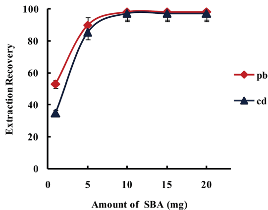
Fig. 5 Effect of amount of SBA-15/Met on the extraction recovery of \text{Pb}^{2+} and \text{Cd}^{2+} with a concentration of 0.1 \mu\text{g L}^{-1} obtained from DSPE-USAEME-SFO. Extraction conditions: similar to those in Fig. 4, except for a sample solution pH of 7.5.
