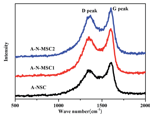
Fig. 5 Raman spectra of different activated HTC carbons as indicated.
