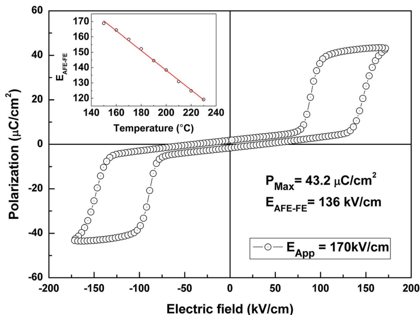
Fig. 10 Polarization vs. electric field ( P - E ) loops for the [111]-oriented plates PLN crystal at 200^{\circ}\text{C} ( f = 10 \text{ Hz} ). Temperature dependence of antiferroelectric parameter of E_{\text{AFE-FE}} for PLN crystal below T_{\text{C}} (inset), showing an ideal linear relationship between temperature and E_{\text{AFE-FE}} .
