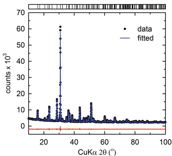
Fig. 3 Rietveld refinement of the powder XRD profile of Sr_2Ca_2MgAl_2Si_3O_{14}:Eu^{2+} . Data (points) and fit (lines), the difference profile, and expected reflection positions are displayed.
