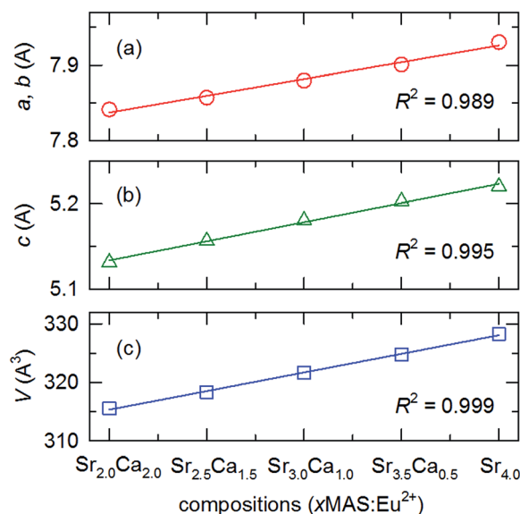
Fig. 4 Variation in lattice parameters (a) a, b , (b) c , and (c) V in SCMAS:Eu^{2+} with variations in cationic ratio. Linear fits of data points corresponding to the Ca^{2+}-Sr^{2+} pair are shown in each plot.
