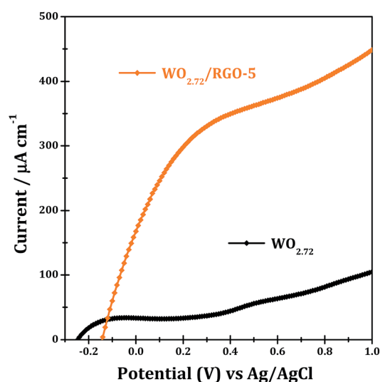
Fig. 13 Photocurrent responses of \text{WO}_{2.72} and \text{WO}_{2.72}/\text{RGO-5} under UV-vis light.
