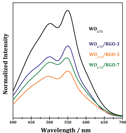
Fig. 12 PL spectra of \text{WO}_{2.72} and \text{WO}_{2.72}/\text{RGO} composites.
