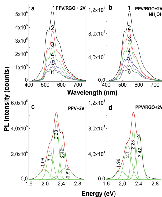
Fig. 8 (a) The PL spectra of the films electro-synthesized onto the Au electrode immersed in the solution of 0.02 \text{ M} TBPX and 0.1 \text{ M} TBAB in \text{DMF} : \text{H}_2\text{O} in the absence (curve 1) and presence of different weight percentage concentrations of RGO, i.e. , 0.01 \text{ wt}\% (curve 2), 0.025 \text{ wt}\% (curve 3), 0.05 \text{ wt}\% (curve 4), 0.1 \text{ wt}\% (curve 5), and 0.5 \text{ wt}\% (curve 6). (b) shows the PL spectra of these films, chemically interacted with the 1 \text{ M} \text{NH}_4\text{OH} solution. The deconvolution of the PL spectra of the films of PPV and PPV/RGO is shown in (c) and (d).
