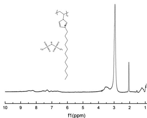
Fig. 9 ^1\text{H-NMR} spectrum of polymeric ionic liquid P1.
