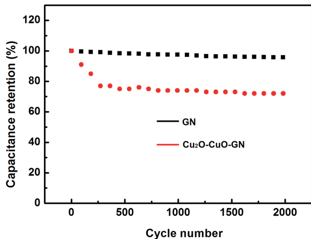
Fig. 6 Comparison of cycle performance of GN and \text{Cu}_2\text{O-CuO-GN} .
