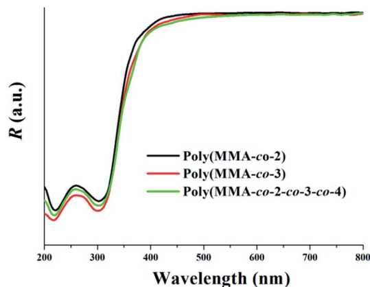
Fig. 5 DR spectra of Poly(MMA-co-2) (200 : 1), Poly(MMA-co-2)@Poly(MMA-co-3)@Poly(MMA-co-4) (1 : 7 : 8) and polymer Poly(MMA-co-2-co-3-co-4) (200 : 1(2/3/4 = 1 : 7 : 8)) in the solid state at room temperature.
