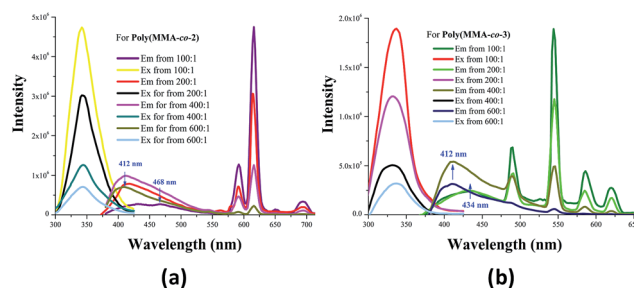
Fig. 6 Emission and excitation spectra ( \lambda_{\text{ex}} = 341 \text{ nm} ) of homo-Ln 3+ -grafted polymers with different feed molar ratios (100 : 1, 200 : 1, 400 : 1 and 600 : 1) in the solid state at room temperature; (6a) for Poly(MMA-co-2); (6b) for Poly(MMA-co-3).
