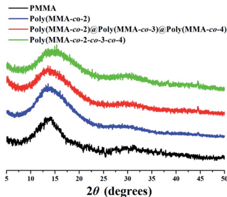
Fig. 3 XRD patterns of PMMA, Poly(MMA-co-2) (200 : 1), polymers' blend Poly(MMA-co-2)@Poly(MMA-co-3)@Poly(MMA-co-4) (1 : 7 : 8) and \text{Eu}^{3+} -Tb ^{3+} -Gd ^{3+} -grafted polymer Poly(MMA-co-2-co-3-co-4) (200 : 1(2/3/4 = 1 : 7 : 8)) in the solid state.
