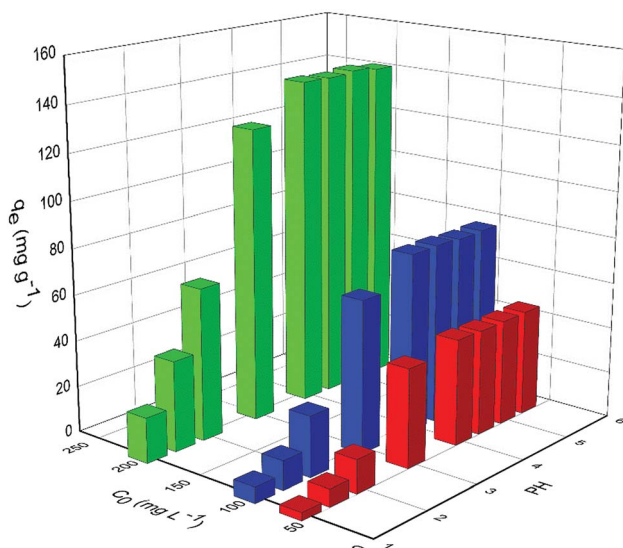
Fig. 5 The effect of initial solution pH on U(VI) removal by PAA hydrogels at various initial concentrations (60, 100 and 200 \text{ mg L}^{-1} ). (Volume, 10 mL; adsorbent dose, 0.01 g; pH value, 1, 1.5, 2, 3, 4, 4.5, 5, 5.5; contact time, 180 min; temperature, 25 \text{ }^\circ\text{C} ; rotating speed, 150 rpm). Note: data are presented as the mean \pm standard deviation of triplicate experiments.
