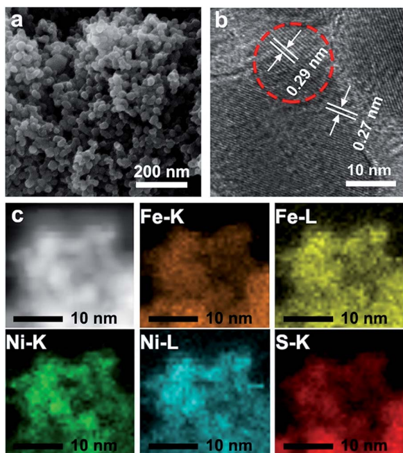
Fig. 1 (a) The SEM image of FeS 2 /NiS nanocomposite. (b) The HRTEM image of FeS 2 /NiS nanocomposite. (c) STEM image and corresponding chemical elements mappings of Fe–K, Fe–L, Ni–K, Ni–L and S–K for FeS 2 /NiS nanocomposite.
