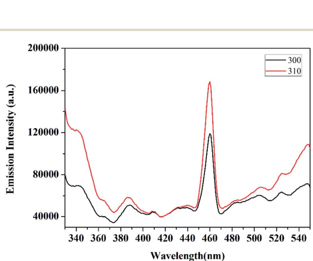
Fig. 4 Photoluminescence (PL) spectra of the \text{CuCrO}_2 nanoparticles, excited at 300 and 310 nm.
