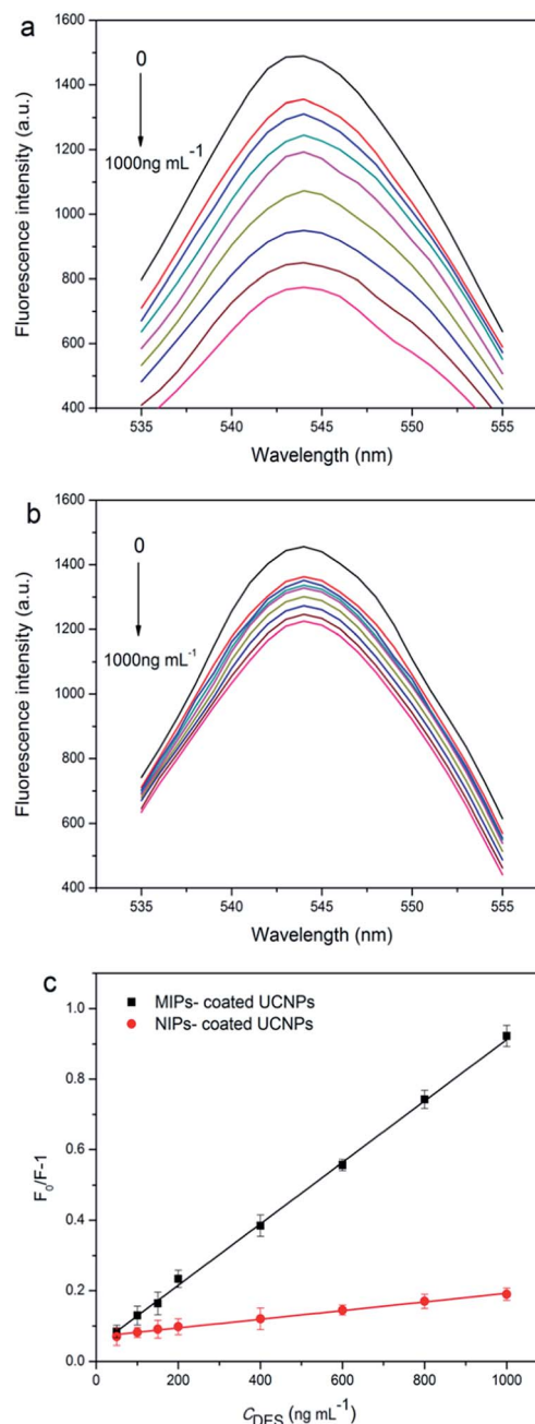
Fig. 4 Fluorescence spectra of MIP-coated UCNP (a) and NIP-coated UCNP (b) with different concentrations of DES; (c) Stern–Volmer curves of DES concentration of MIPs-coated UCNP and NIPs-coated UCNP.
