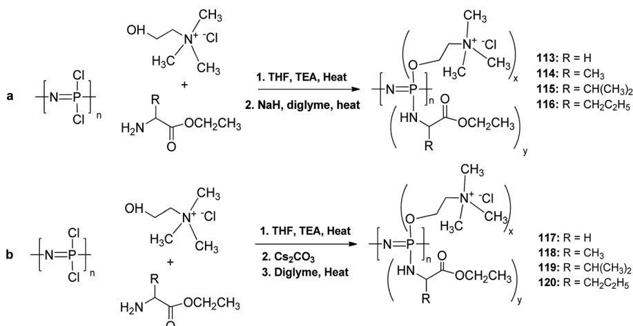
Scheme 27 Synthesis of poly[(amino ethyl ester),(choline chloride),phosphazene] using two different routes: (a) sodium hydride (NaH) (113–116), (b) cesium carbonate ( \text{Cs}_2\text{CO}_3 ) (117–120). 145
