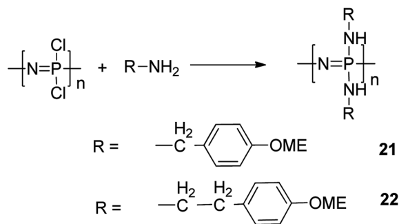
Scheme 5 Synthesis of aromatic groups attached through nitrogen. 56
