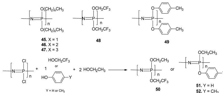
Scheme 9 Single-substituent polymers (45–49) and polymers with both ethoxy and O-linked co-substituents (50–52). 45
