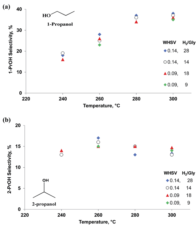
Fig. 6 Selectivity vs. temperature for (a) 1-PrOH and (b) 2-PrOH at \text{WHSV} = 0.09 to 0.14 \text{ h}^{-1} , residence time = 0.43 \text{ s} and 0.65 \text{ s} and \text{H}_2/\text{gly} ratio = 9, 14, 18 and 28 .
