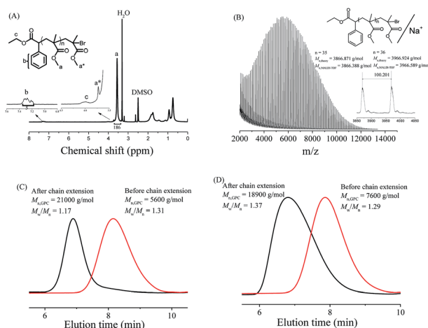
Fig. 2 ^1\text{H} NMR spectrum (A) and MALDI-TOF MS (B) of the resultant PMMA. Polymerization conditions of sample PMMA ( M_{n,GPC} = 6900 g \text{mol}^{-1} , M_{n,NMR} = 6400 g \text{mol}^{-1} , M_w/M_n = 1.35 ): [\text{MMA}]_0 : [\text{EBPA}]_0 : [\text{FeBr}_2]_0 = 100 : 1 : 1 , V_{\text{MMA}} = 1.0 mL, V_{\text{DMI}} = 0.5 mL, time = 15 h, at room temperature under UV irradiation ( 900 \mu\text{W cm}^{-2} ) at 360 nm. GPC traces of PMMA before and after chain extension under both photo-induced (C) and thermal (D) conditions. Chain extension conditions via photochemical reaction: [\text{MMA}]_0 : [\text{PMMA}]_0 : [\text{FeBr}_2]_0 = 100 : 0.4 : 1 , V_{\text{MMA}} = 1.0 mL, V_{\text{DMI}} = 0.5 mL, time = 54 h, at room temperature under UV irradiation ( 900 \mu\text{W cm}^{-2} ) at 360 nm. Chain extension conditions via thermal polymerization reaction: [\text{MMA}]_0 : [\text{PMMA}]_0 : [\text{Fe}(\text{acac})_3]_0 : [\text{PPh}_3]_0 : [\text{AsAc}]_0 = 100 : 0.4 : 1 : 3 : 4 , V_{\text{MMA}} = 1.0 mL, V_{\text{toluene}} = 1.0 mL, T = 70^\circ\text{C} , time = 24 h.
