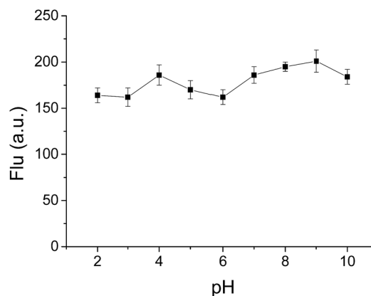
Fig. 5 Fluorescence intensity of BBTA in \text{H}_2\text{O} -mPEG 550 (95 : 5, v/v, 10 \mu\text{M} ) with different pH (error bar represents standard deviation). \lambda_{\text{ex}} = 405 \text{ nm} .
