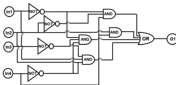
Fig. 11 Combinational logic circuits equivalent to the truth table given in Table 1: In1 (UV), In2 (Vis), In3 ( Hg^{2+} ), In4 (Cys).
