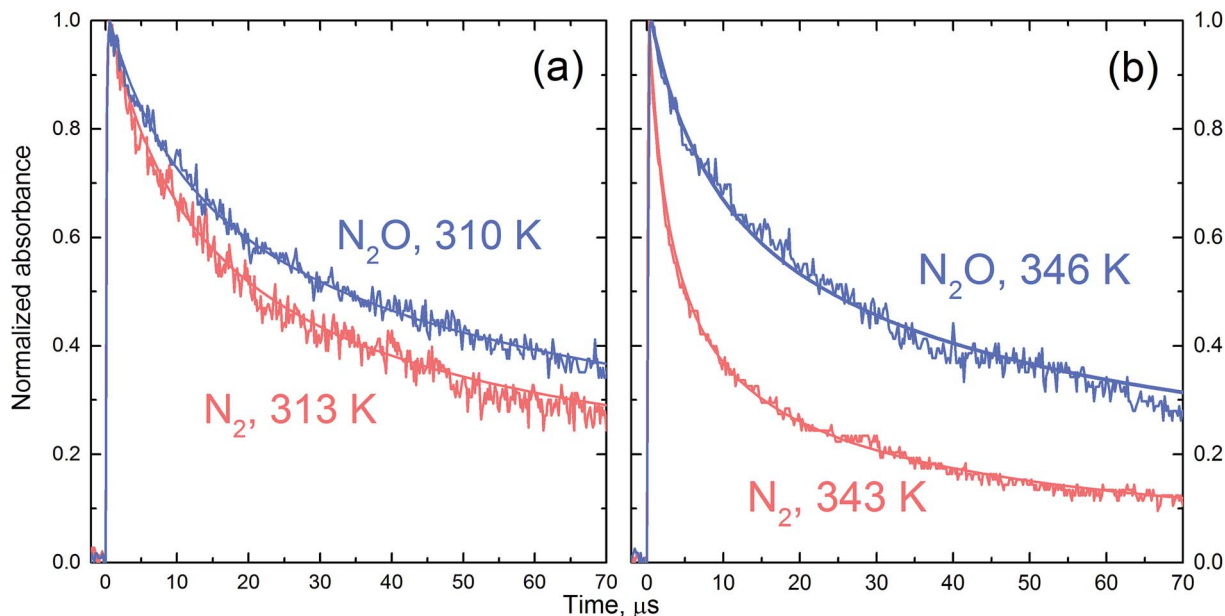
Fig. 3 The normalized-to-maximum transient absorbance of \text{Cl}_2^{*\cdot-} in pulse irradiated aqueous 0.1 M HCl solution saturated with \text{N}_2 (pink) and \text{N}_2\text{O} (blue) recorded at 340 nm after 7 ns pulse at ca. 313 K (a) and 343 K (b). The solid lines through the experimental traces present FACSIMILE fits obtained taking into account the reaction set from Table 2, and allowing k'_{\text{R1}} to vary.
