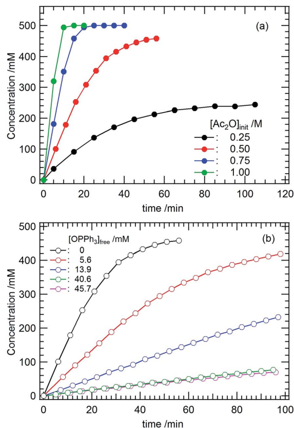
Fig. 3 The progress of the acetylation of \text{Ph}(\text{CH}_2)_2\text{OH} catalyzed by [\text{UO}_2(\text{OPPh}_3)_4]^{2+} ( 4 ) in \text{CD}_2\text{Cl}_2 at 22 °C. (a) [\text{Ac}_2\text{O}] dependency; initial condition: 0.50 M \text{Ph}(\text{CH}_2)_2\text{OH} , 0.25–1.00 M \text{Ac}_2\text{O} and 6.5 mM 4 , and (b) [\text{OPPh}_3] dependency; initial condition: 0.50 M \text{Ph}(\text{CH}_2)_2\text{OH} , 0.50 M \text{Ac}_2\text{O} , 6.5 mM 4 and 0–45.7 mM \text{OPPh}_3 .
