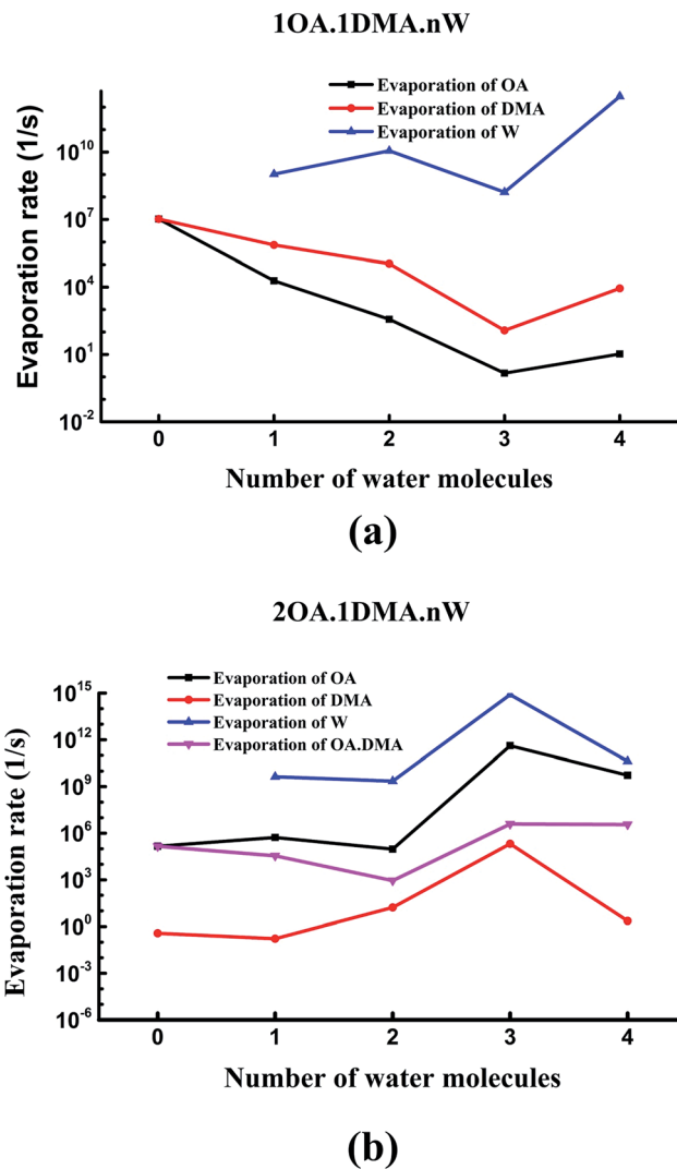
Fig. 7 Evaporation rates of oxalic acid, dimethylamine and water molecules from (C 2 H 2 O 4 )(CH 3 NHCH 3 )(H 2 O) n ( n = 0-4 ) clusters (a), and (C 2 H 2 O 4 ) 2 (CH 3 NHCH 3 )(H 2 O) n ( n = 0-4 ) clusters (b).
